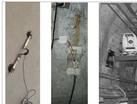
Fig 2: Various sensors installed for assessing data.
